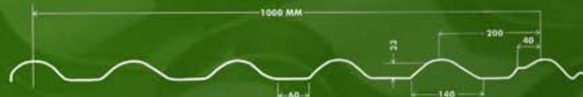
SECTION DRAWING
