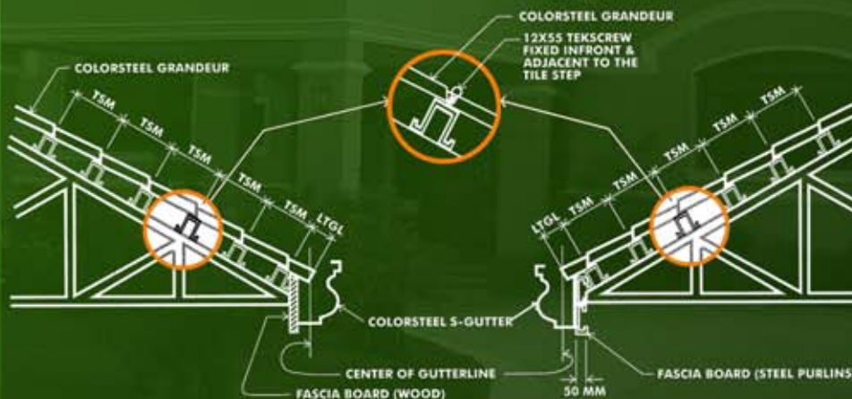
INSTALLATION SET-UP NO. 1
